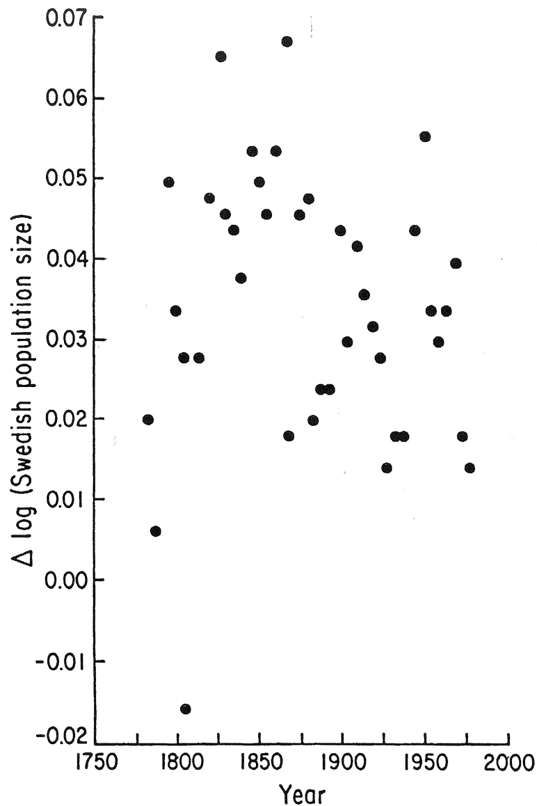
Figure 1. — Forward first differences of the natural logarithm of Swedish total population size (in thousands) from 1780 to 1975. NOTE: If Z(t) is the total population size (in thousands) at one point of observation and Z(t + 1) is the total population size (in thousands) at the next quinquennium, then the ordinate is \log Z(t + 1) - \log Z(t) .
