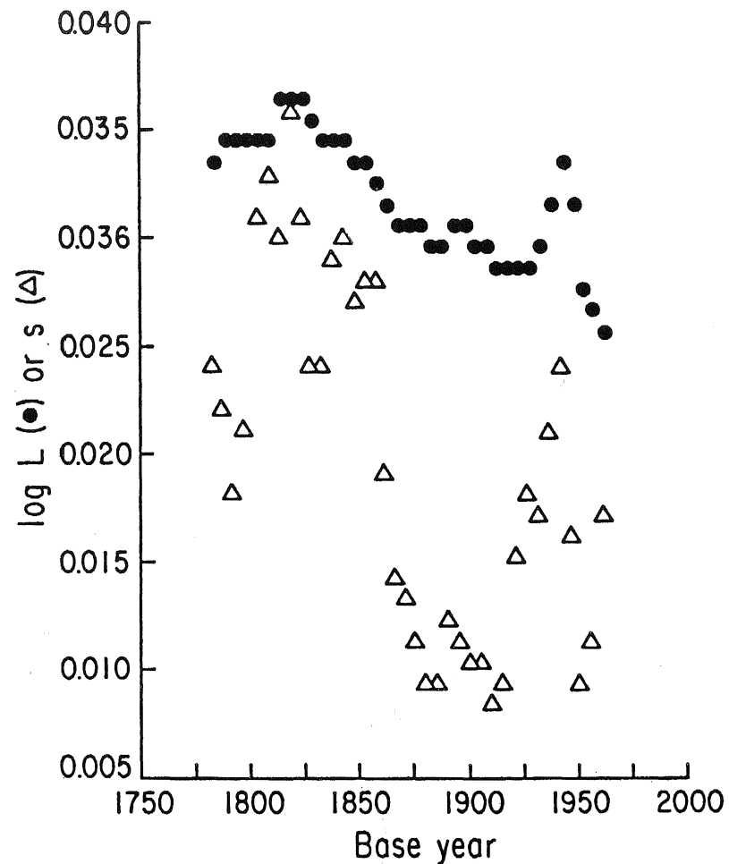
Figure 2. — Estimated growth rates ( \log L ) and coefficients of dispersion ( s ) for Swedish population projections with a launch of 1980 and various base years. NOTE: \log L from equation (2); s from equation (3). Population in thousands, observed at quinquennial intervals.
