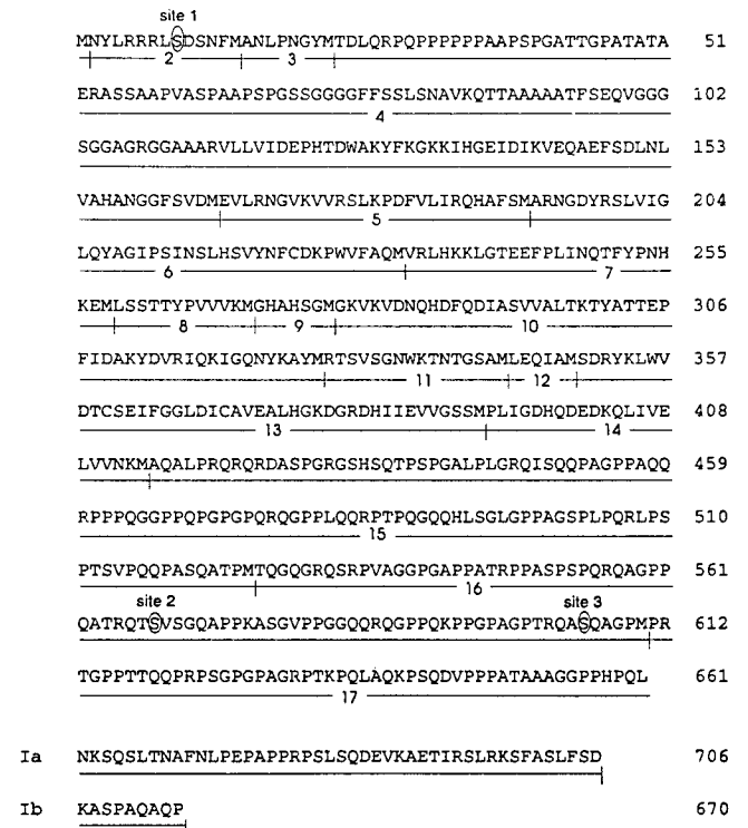
Fig. 3. Amino acid sequences of synapsin Ia and Ib. The CNBr cleavage sites are indicated together with the resulting fragments numbered from 1 to 17. The circled serines are the sites of phosphorylation (see text).
