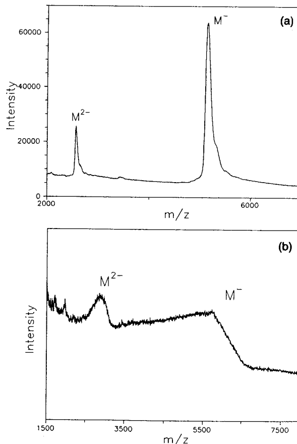
Figure 8. Negative-ion mass spectra of (a) d(\text{uridine})_{18} and (b) d(\text{inosine})_{18} from ferulic acid.
