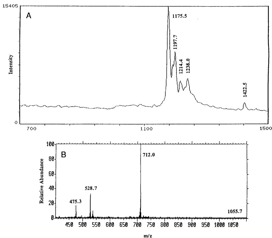
Fig. 3. Mass spectra of cystine peptides P2a and P3a obtained from thermolytic digestion of Er-2 . Peptide P2a (A) was analyzed by matrix-assisted laser desorption mass spectrometry on a time-of-flight mass spectrometer as described under Materials and methods. Peptide P3a (B) was brought to a concentration of 5 pmol/ \mu L with H 2 O:CH 3 OH:acetic acid (45:50:5) and analyzed by electrospray mass spectrometry.
