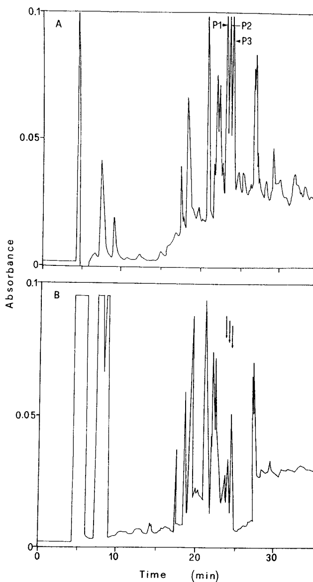
Fig. 1. Reverse-phase HPLC profiles of unreduced and reduced aliquots of thermolysin-digested Er-2. Native Er-2 was digested with thermolysin for 24 h. Two equivalent aliquots ( \frac{1}{2} of the total digest) were removed. One (A) was untreated and the other (B) was treated with 0.1% \beta -mercaptoethanol in 0.2 M Tris, pH 8.5, for 5 h. Both samples were analyzed by microbore reverse-phase HPLC on a C18 column (2.1 \times 220 mm) utilizing \text{CH}_3\text{CN}:\text{H}_2\text{O} (4:1) containing 0.08% TFA as the mobile phase. The peptides were eluted with a linear gradient and detected by their absorbance at 214 nm as described under Materials and methods. P1, P2, and P3 were the only peaks that contained detectable cystine after acid hydrolysis.
