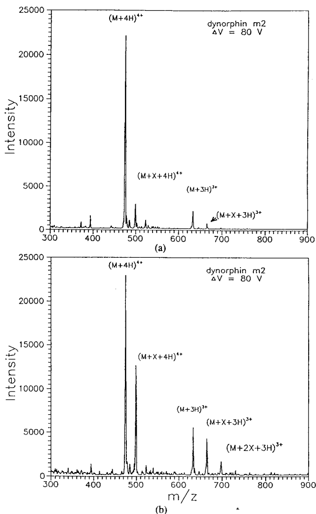
Figure 4. Electrospray ionization of dynorphin model 2 dissolved in a mixture of water, methanol, and acetic acid (47:50:3 v/v). Concentration = 2.0 pmol/ \mu L; flow rate = 0.7 \mu L/min. Each of the spectra is a single scan acquired in 57 s. V(\text{skimmer}) = 20 V, \Delta V = 80 V. (a) no salt added; (b) 40 pmol/ \mu L ammonium sulfate added.
