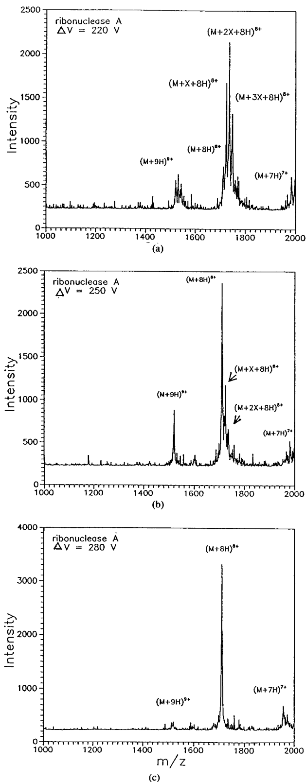
Figure 3. Electro spray ionization spectra of bovine pancreatic ribonuclease A obtained from a solution of water, methanol, and acetic acid (48.5:48.5:3.0 v/v). Concentration = 10 pmol/ \mu L, flow rate = 0.5 \mu L/min. Each spectrum is an average of five scans, requiring 145 s/scan. Thus, 60 pmol of ribonuclease A was consumed in acquiring each of the spectra. V(\text{skimmer}) = 20 V. (a) \Delta V = 220 V; (b) \Delta V = 250 V; (c) \Delta V = 280 V. Data was obtained to m/z 2000, the upper limit of the mass spectrometer.
