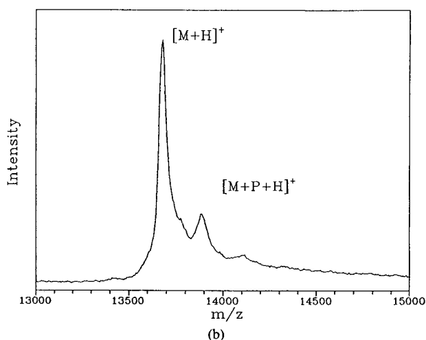
Figure 6. The matrix assisted laser desorption mass spectrum of bovine ribonuclease A using sinapinic acid matrix. From (a) the untreated protein sample and (b) after treatment with barium acetate.
