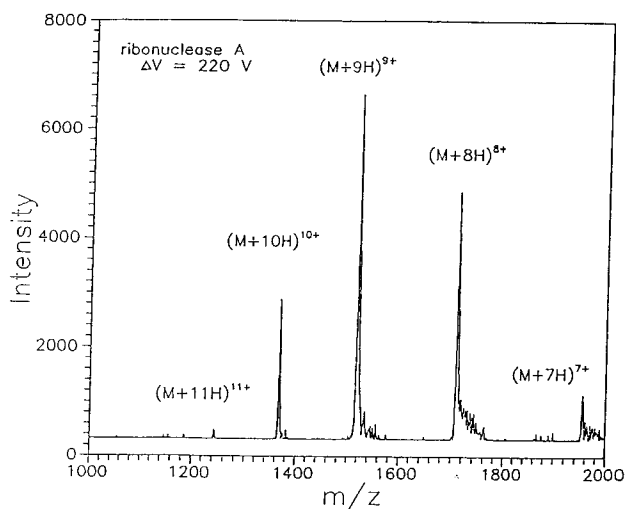
Figure 5. Electrospray ionization spectra of bovine pancreatic ribonuclease A after treatment with barium acetate. All other conditions are the same as those given in the caption for Figure 3a.
