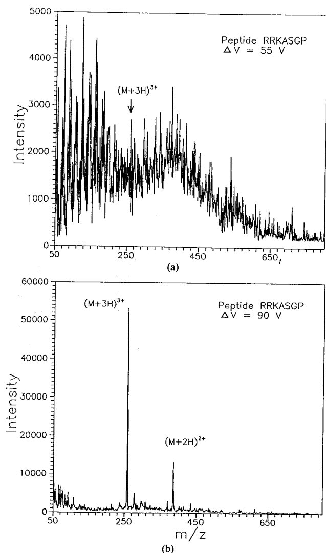
Figure 2. Electrospray ionization spectra of the peptide RRKASGP, measured at two different values of the potential difference ( \Delta V ) applied between the capillary tube and the skimmer. The temperature of the tube is \sim 85^\circ\text{C} and the potential applied to the skimmer, V(\text{skimmer}) = 20\text{ V} . (a) \Delta V = 55\text{ V} ; (b) \Delta V = 90\text{ V} . The spectra are single scans, each acquired in 62 s. Each data point in the scan is averaged three times by the data system.
