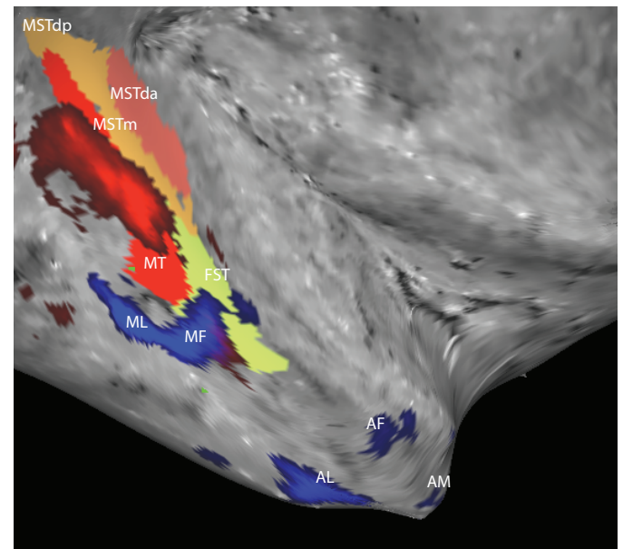
Motion (red) p > 10^{43} Faces (blue) p > 10^{45}
