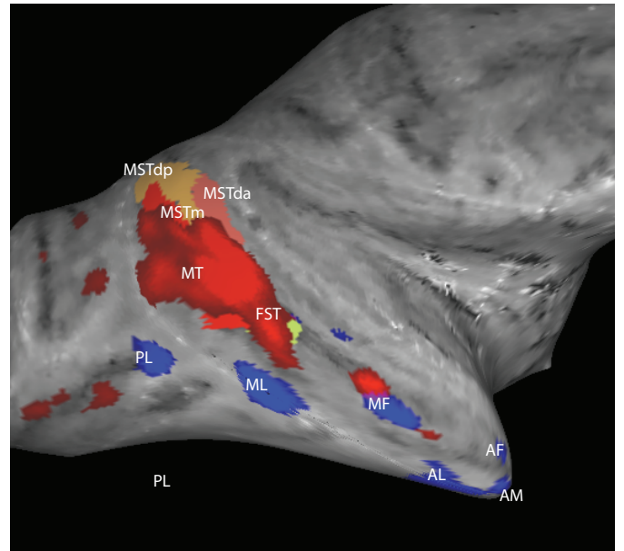
Motion (red) p > 10^{35} Faces (blue) p > 10^{42}
