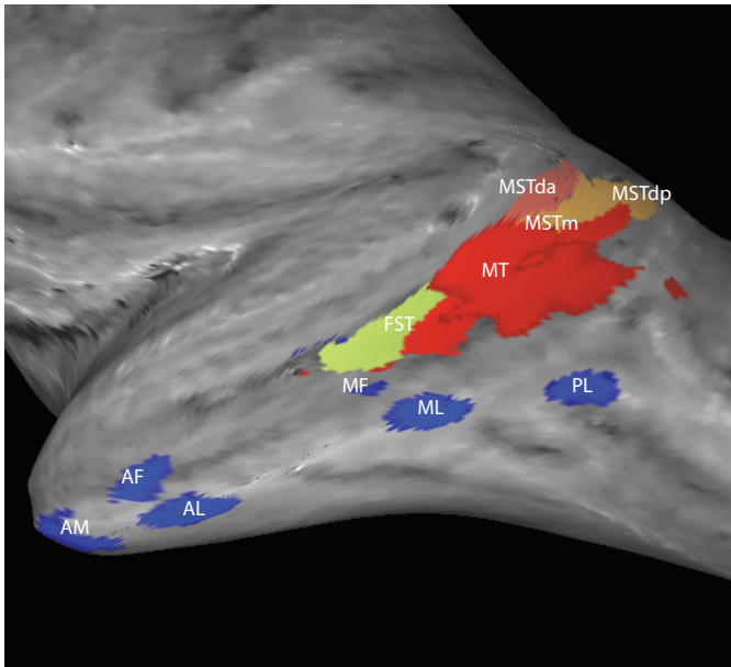
Motion (red) p > 10^{50} Faces (blue) p > 10^{43}
