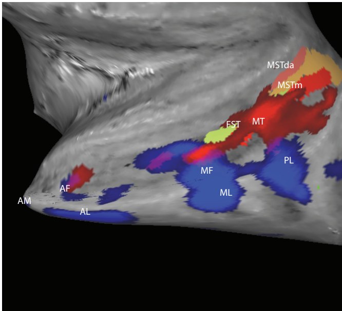
Motion (red) p > 10^{30} Faces (blue) p > 10^{44}
