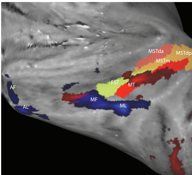
Motion (red) p > 10^{44} Faces (blue) p > 10^{44}
