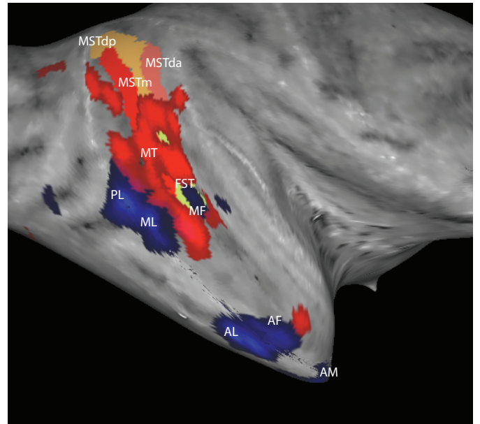
Motion (red) p > 10^{25} Faces (blue) p > 10^{47}
